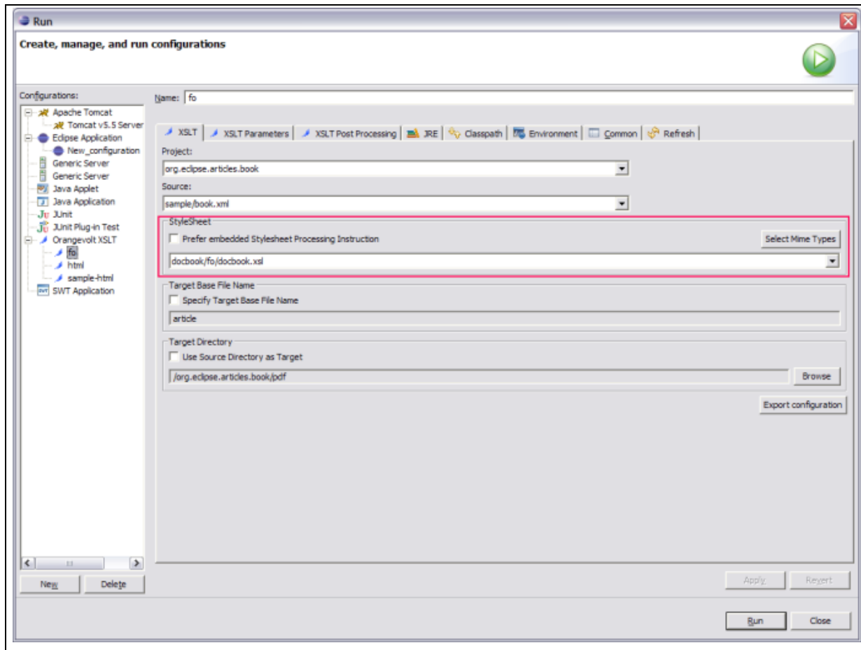
Figure 3. Sample XSL-FO Transformation Configuration for book.xml
